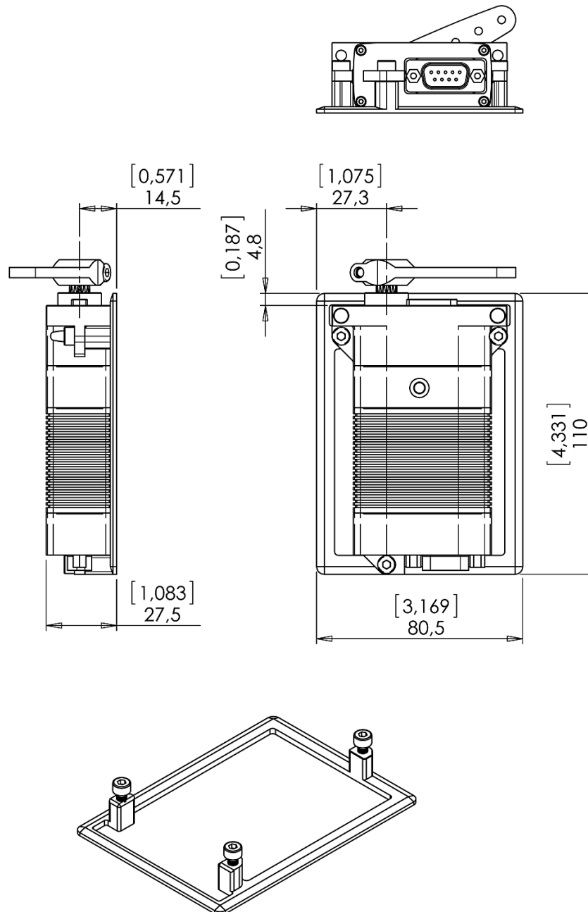
Mounting Frame shown with installed actuator.
